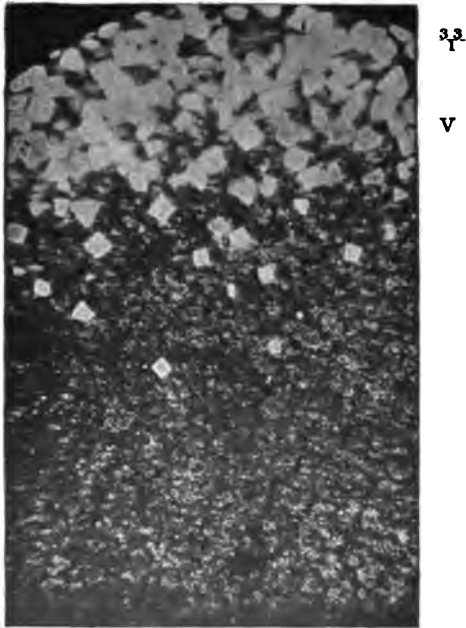
Fig. 16. Alloy of 90 per cent Tin, 10 per cent Antimony. Showing how the Cubes of Tin Antimonide (Sn Sb) have risen by Gravity to the Top of the Ingot. Vertical Section of the Ingot. Prepared by William Campbell in the Author's Laboratory.
